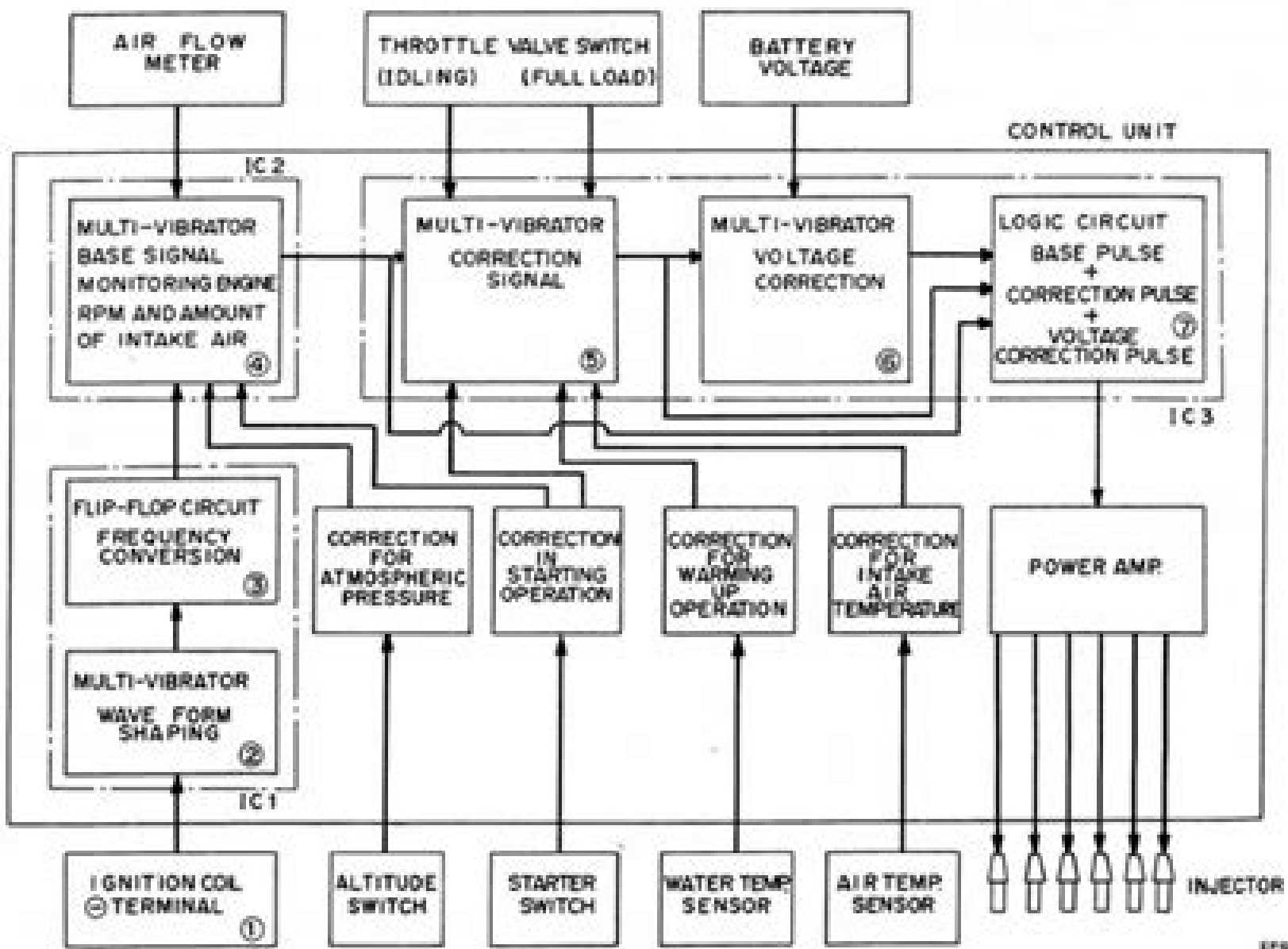
Fig. EP-1 Control unit block diagram
