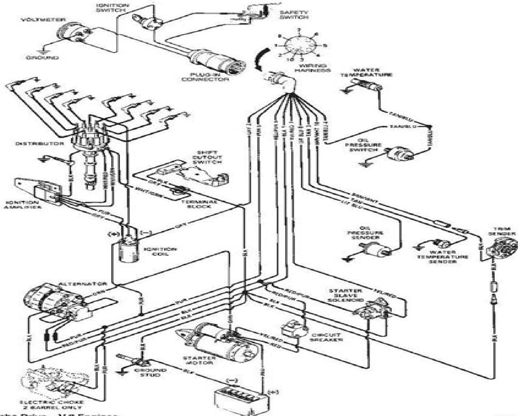
Typical Alpha Drive - V-8 Engines
