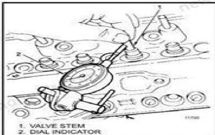
FIGURE 2. VALVE STEM CLEARANCE
