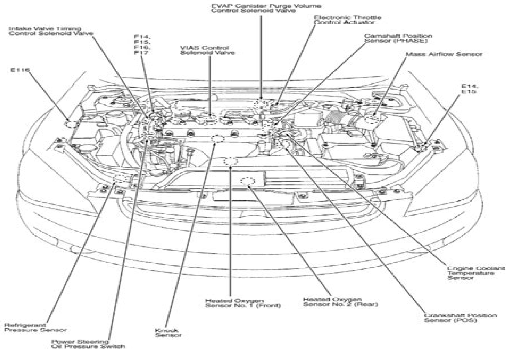
Fig 1: Engine Compartment (2.5L VIN A)
