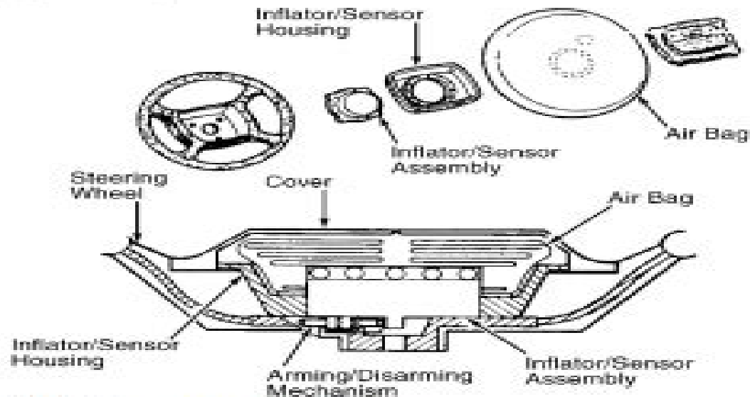
91012508 Fig. 1: Identifying Driver-Side Air Bag Module Components Courtesy of Jaguar Cars, Inc.
