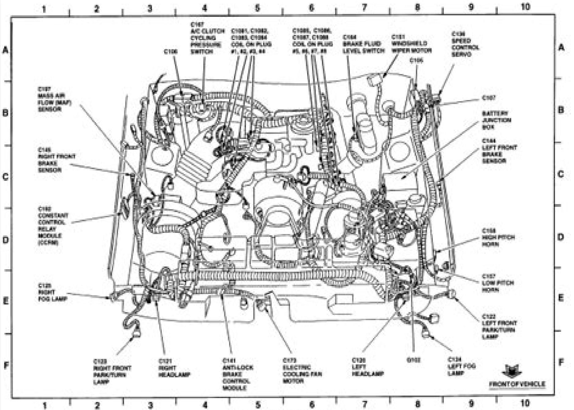
4.6L 2V ENGINE (1 OF 3)
