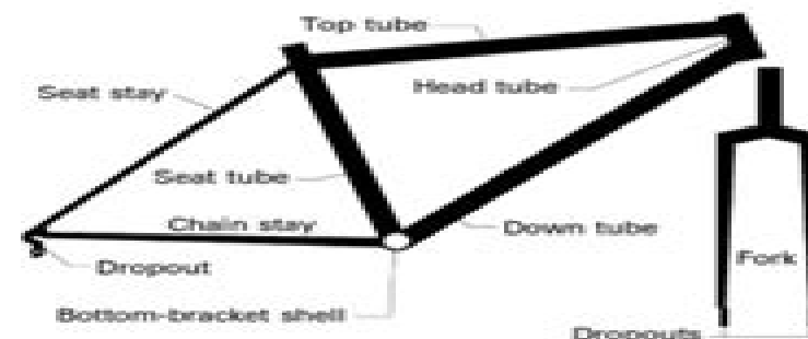
1.1 Parts of the frame.
