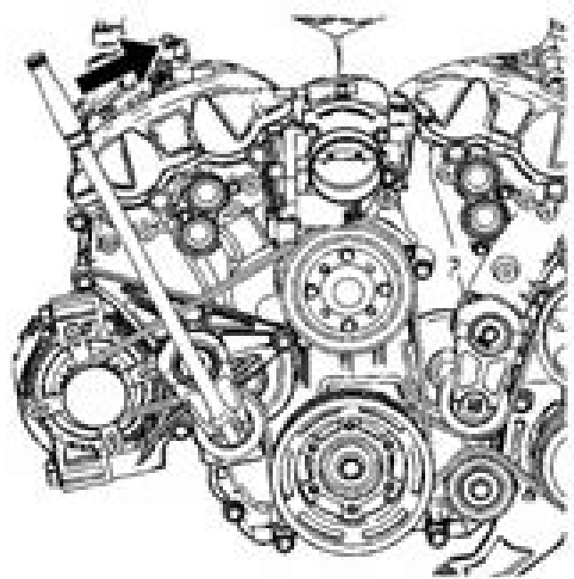
Fig. 1: Removing/Installing Generator & Water Pump Drive Belt Courtesy of GENERAL MOTORS CORP.
