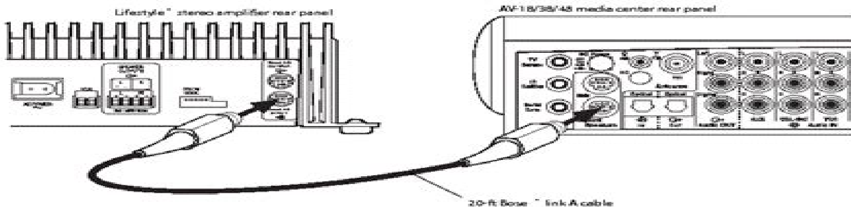
Figure 5 Lifestyle™ stereo amplifier to AV-18/38/48 media center connections
