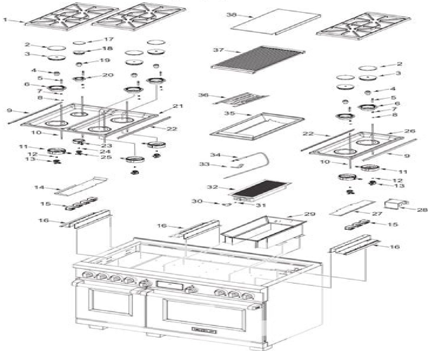
48" Dual Fuel Range Top Exploded View for DF486C
