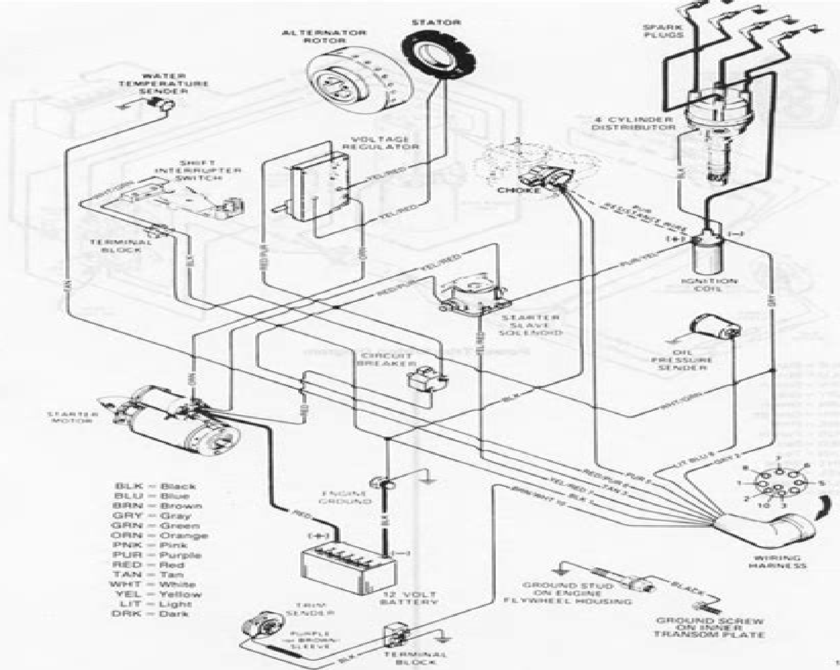
Engine Electrical System Wiring Diagram
