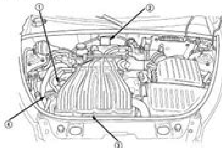
Fig. 9 Coolant Recovery Container and Pressure Cap
