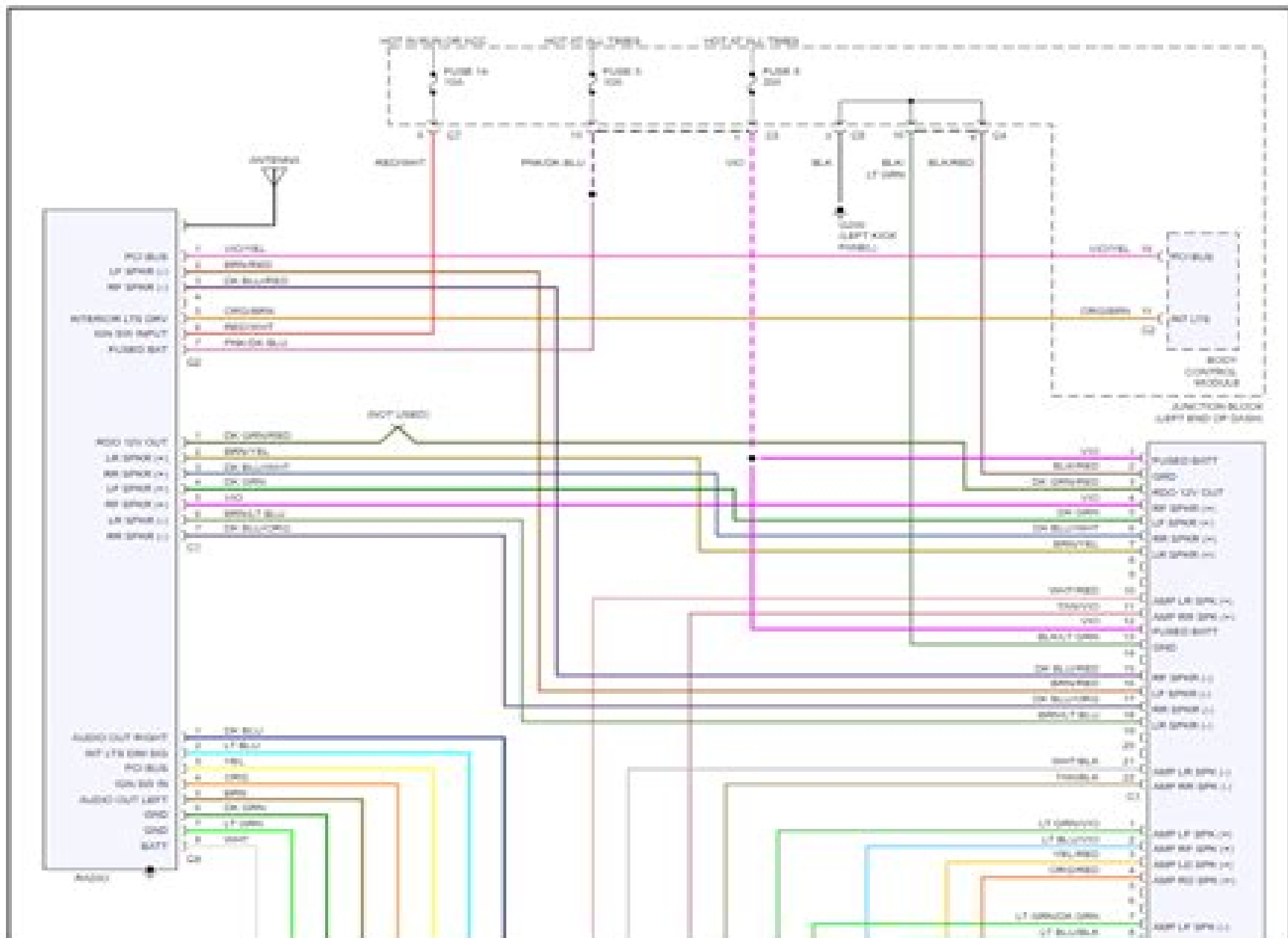
Fig 2: Radio Circuit, Premium Radio
