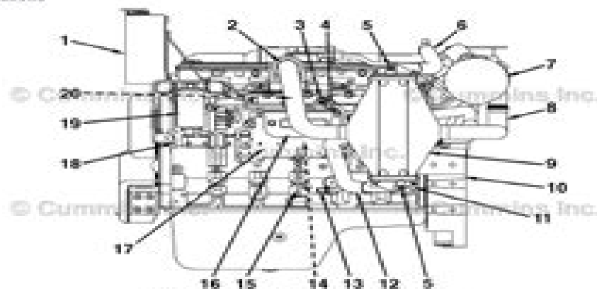
Left View (Port) QSL9 Marine (Keel Cooled)
