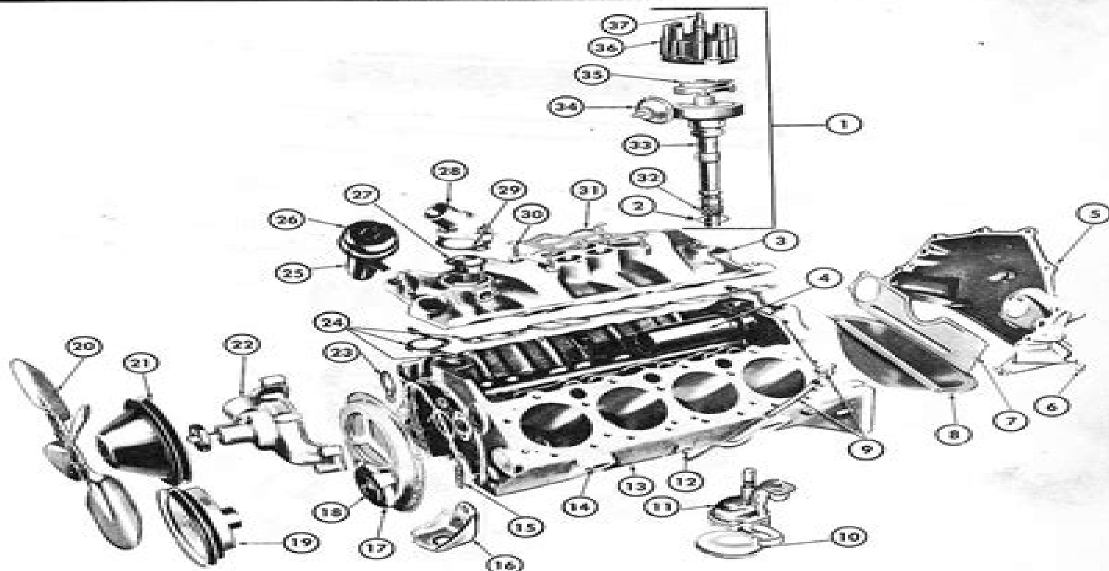
ENGINE BLOCK—8 CYL. ENGINE (TYPICAL)
