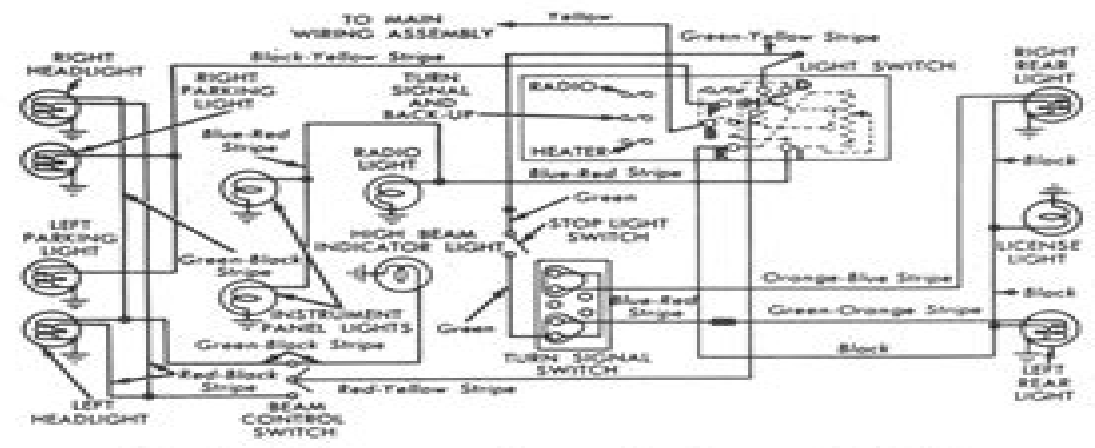
Exterior & Instrument Lamp Circuits . . 1961-62
