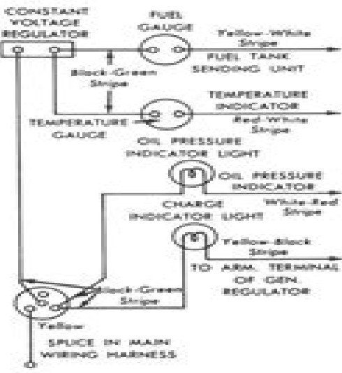
Instrument Gauge Circuit . . 1961-62
