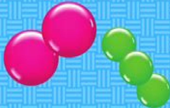
Molecules
