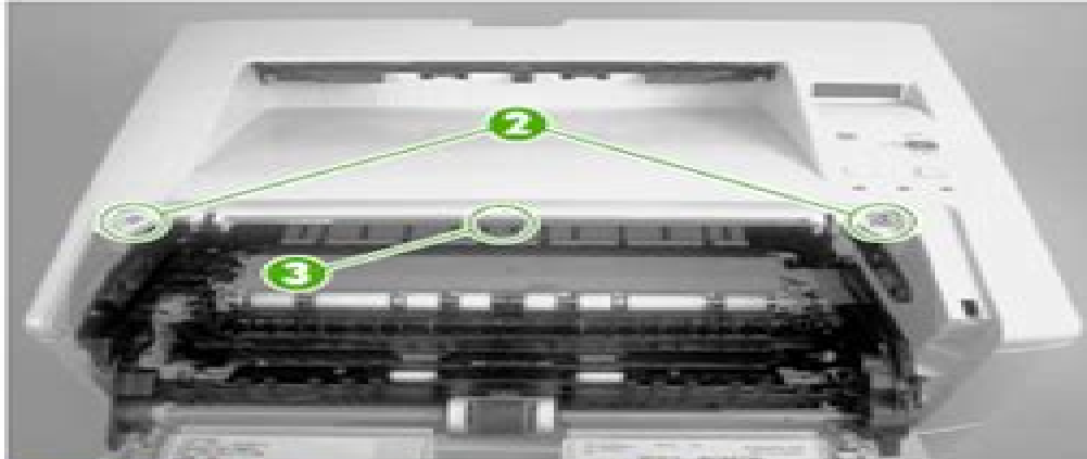
Figure 5-46 Removing the top cover (2 of 5)
