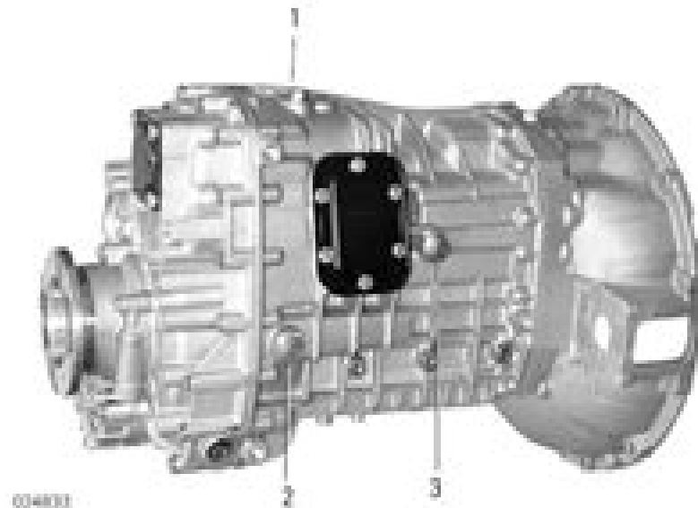
Fig. 11 Position of oil plugs (viewed from below) shown on model series 9 S 1110
