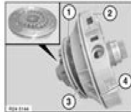
Fig. 34. Identifying Installation Position Of Gears Courtesy of BMW OF NORTH AMERICA, INC.
