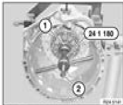
Fig. 32. Removing Oil Supply Vent From Transmission Housing Using Special Tool 24.1.180 Courtesy of BMW OF NORTH AMERICA, INC.
