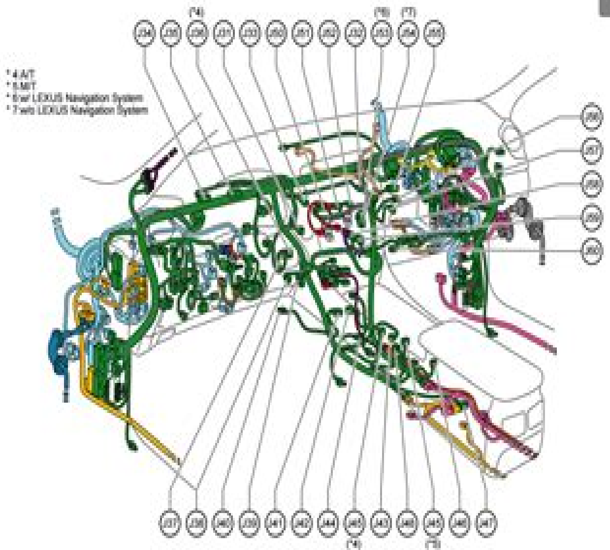
Position of Parts in Instrument Panel (1/10)
