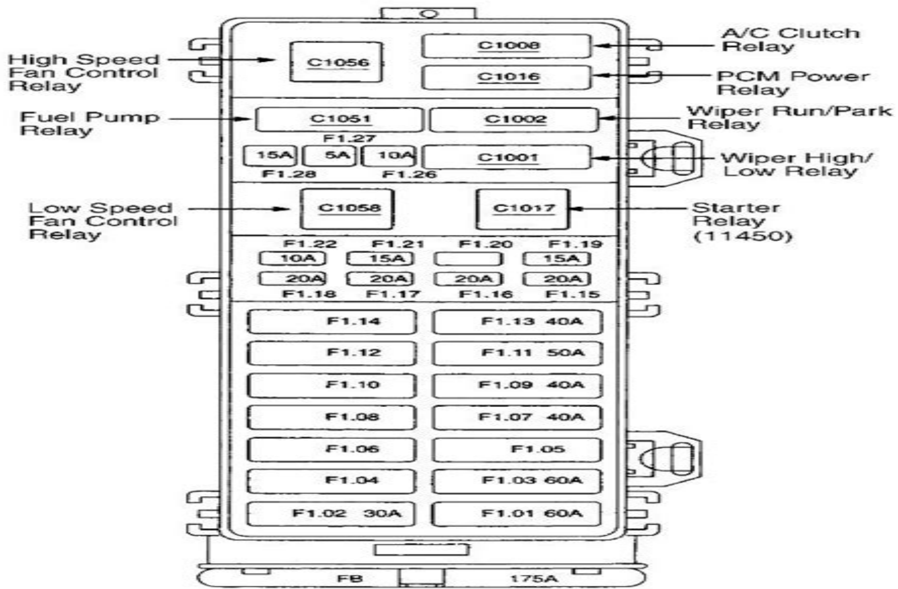
Fig 2: Identifying Battery Junction Box Components
