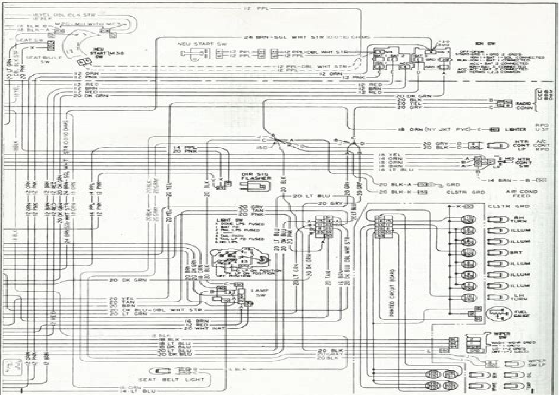
Fig. 81—Instrument Cluster (Nova)
