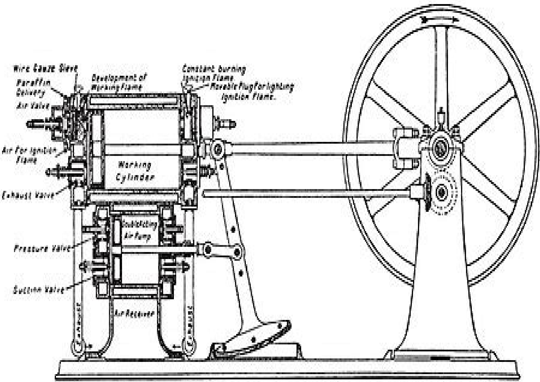
FIG. 2.—Brayton petrol engine. A.D. 1876. (Longitudinal section.)
