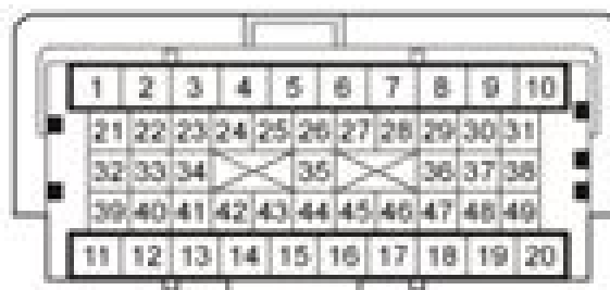
Terminal side of male terminals
