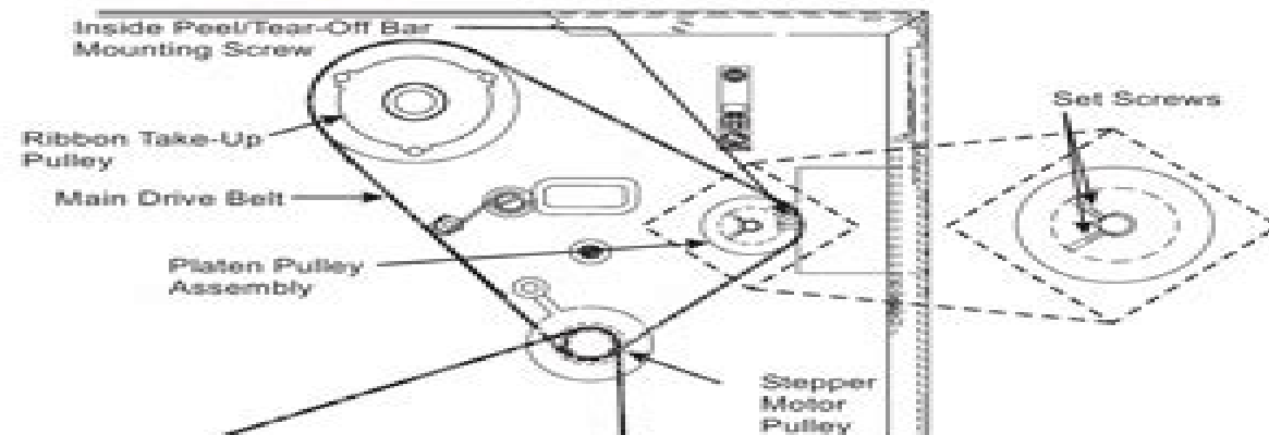
Figure 4-28. Replace the Platen Pulley
