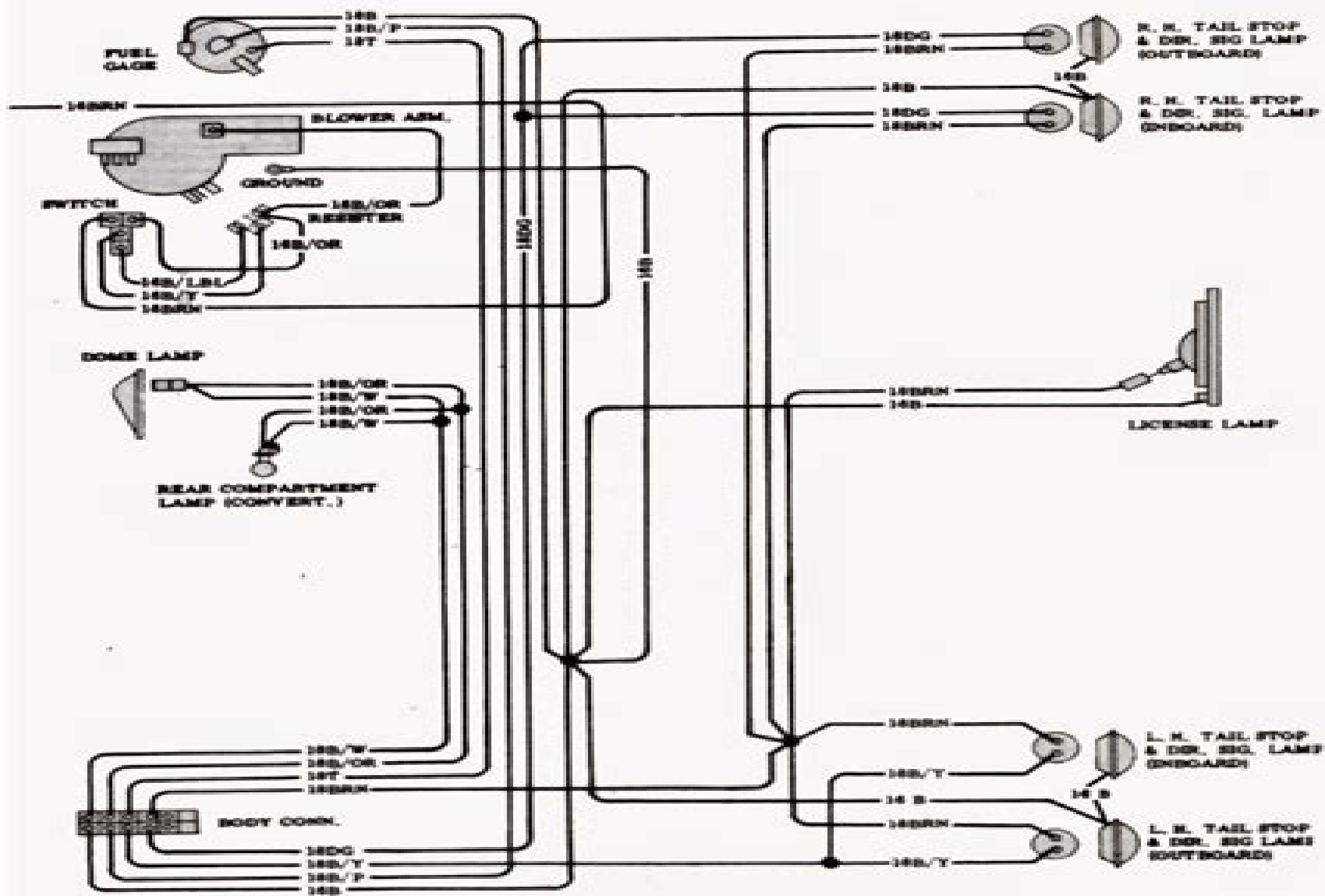
Body and tail lamp wiring, Corvette, 1965.
